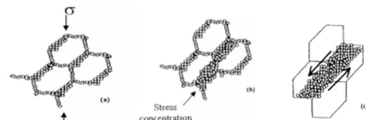
Figure 2. Twin induced heterogeneous recrystallization leading to shear banding and hot cracking in coarse-grained commercial Mg alloys (Ion1982).
