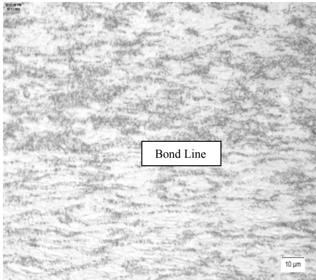
Figure 6. Bond line in TTMP stack rolled AZ6/1.8 on 260°C rolls.
